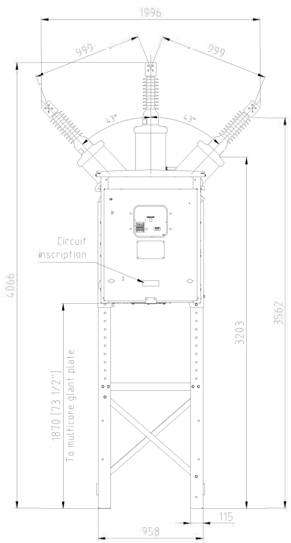
FRONT VIEW SUPPORT AT MAXIMUM HEIGHT
