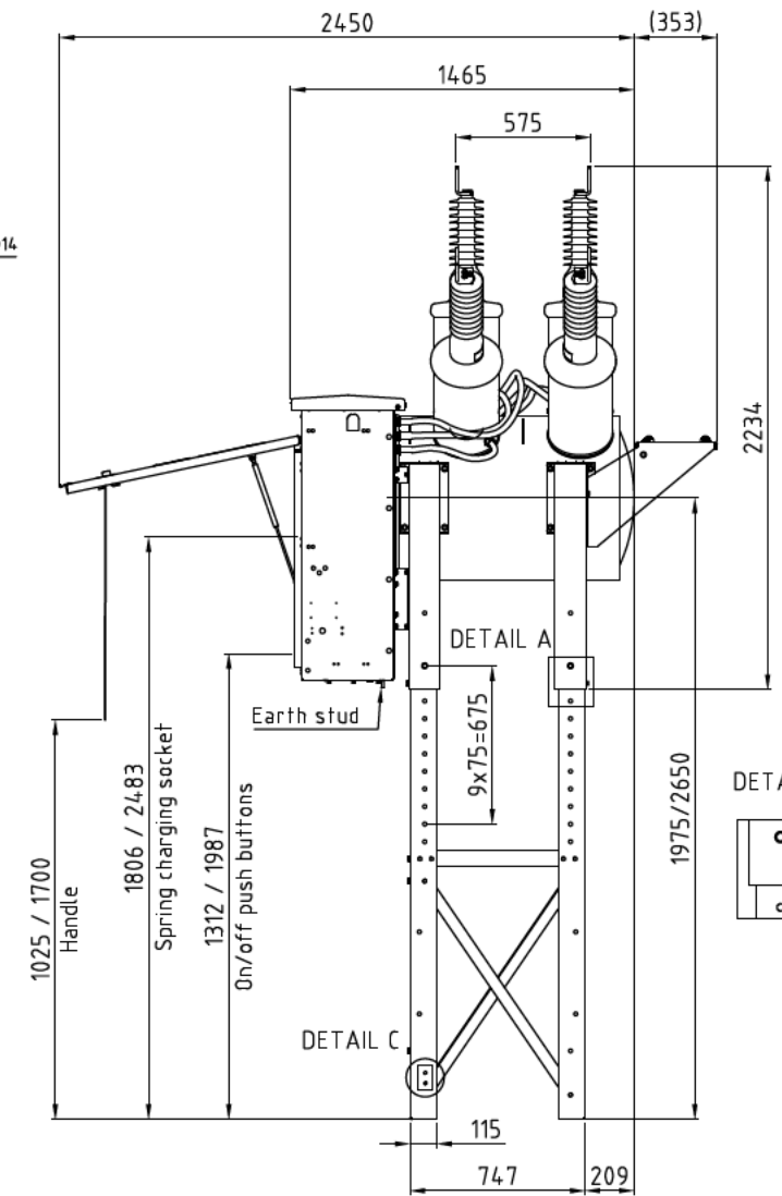
SIDE VIEW AT MAXIMUM HEIGHT (DIMENSIONS GIVEN FOR SUPPORT AT MIN/MAX HEIGHT)
