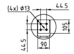
DETAIL B (1:8)
