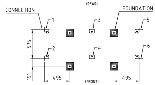
POSITION FOUNDATION / CONNECTION TOP VIEW
