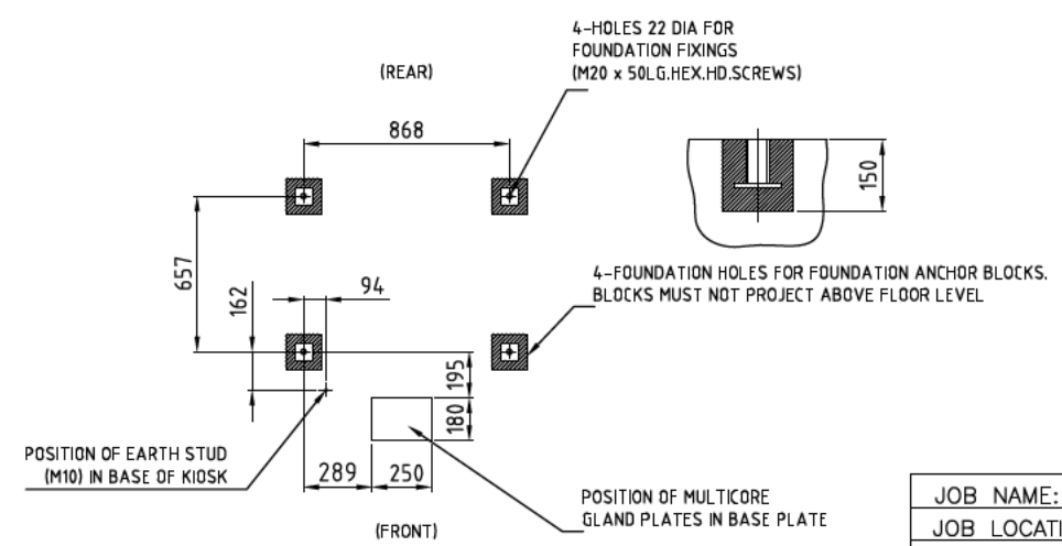
FOUNDATION PLAN TOP VIEW
