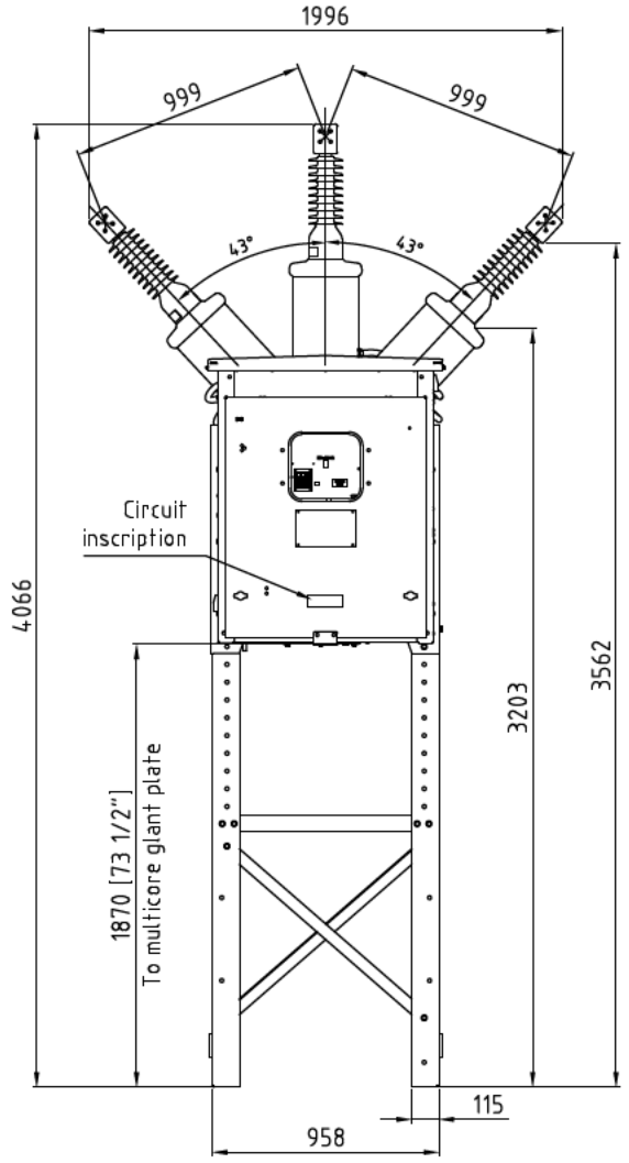
FRONT VIEW SUPPORT AT MAXIMUM HEIGHT
